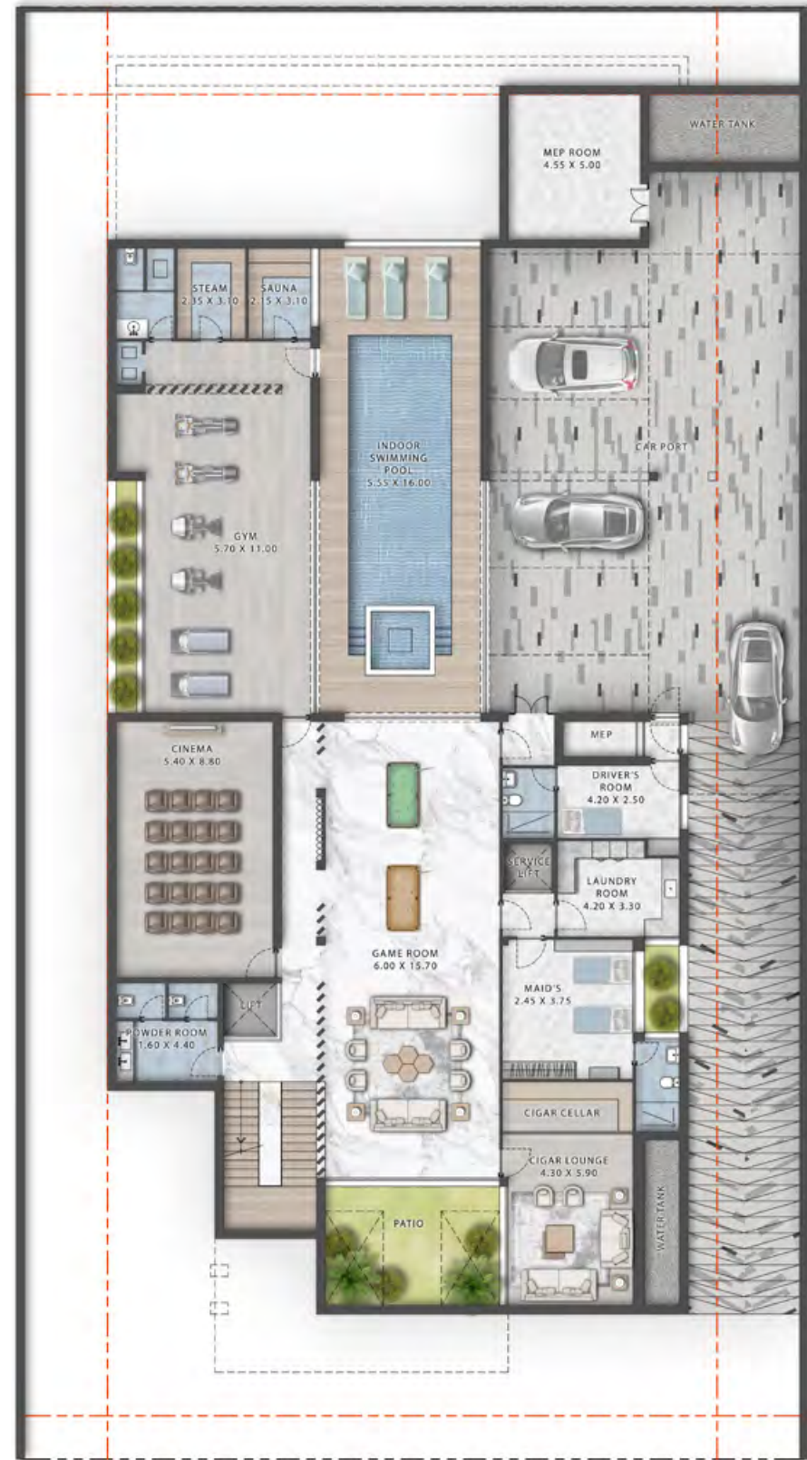
BASEMENT FLOOR
