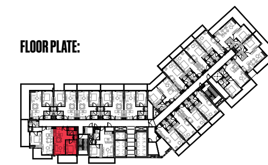
Floors 03 - 09
